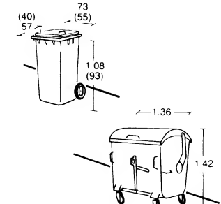
⑮ Large bins (intermediate waste containers)
